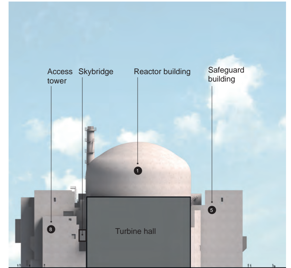
Figure 7.12: Nuclear island unit 2 buildings east elevation, at 1:1250
