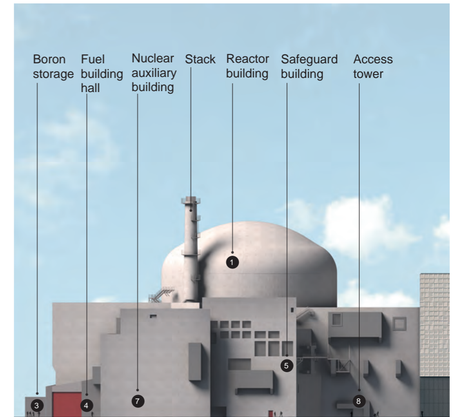
Figure 7.13: Nuclear island unit 2 buildings south elevation, at 1:1250
