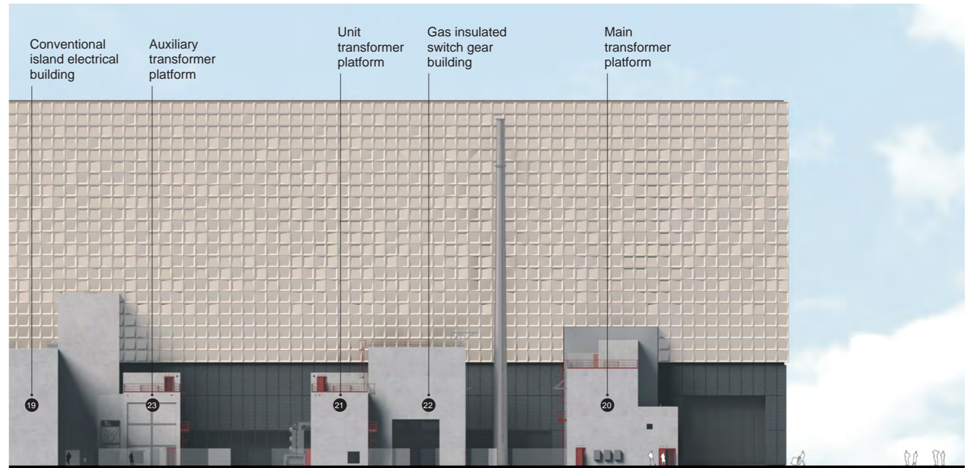
Power transmission platform
