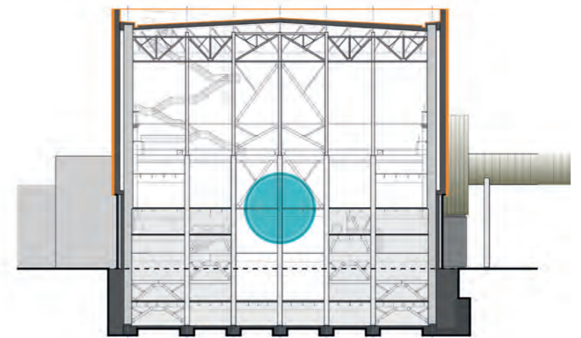
Figure 7.24: Turbine hall diagrammatic connections in section
