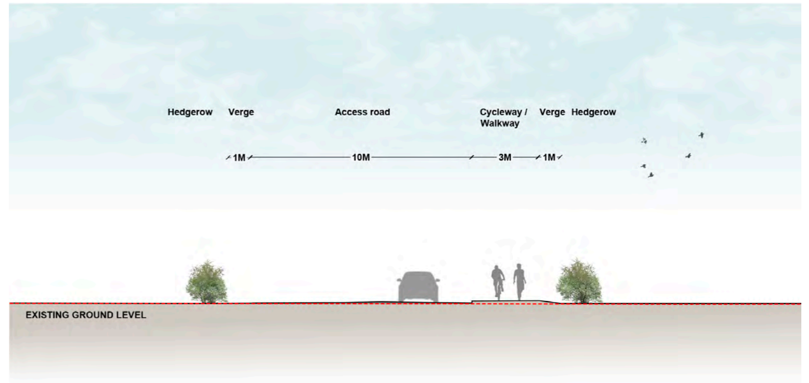
Section O-O'
